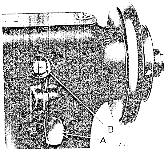
Fig. 17. Stitch Regulator
