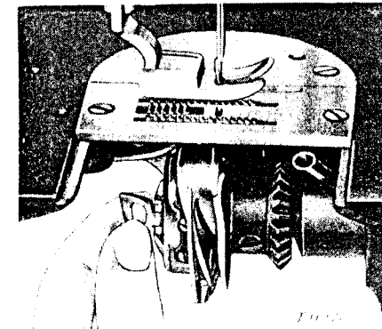
Fig. 8. Removing the Bobbin Case
