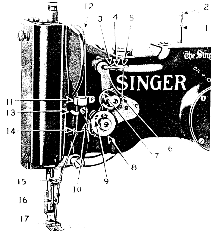
Fig. 13. Threading the Needle
