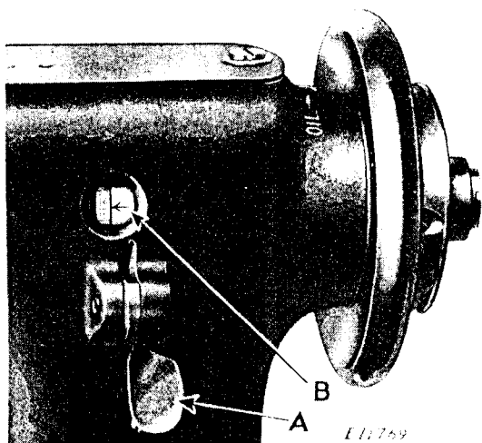
Fig. 17. Stitch Regulator
