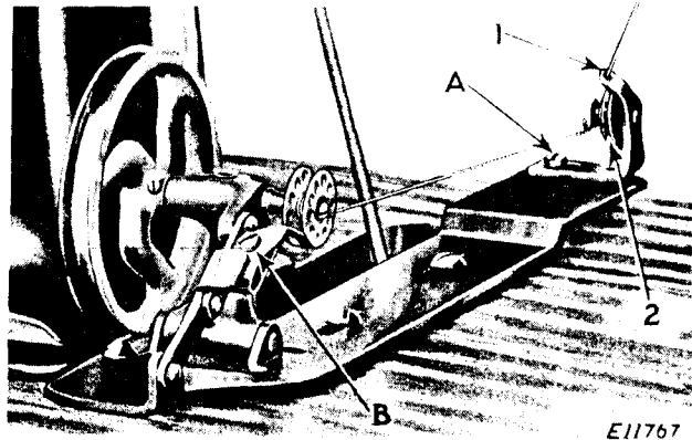
Fig. 9. Winding the Bobbin
