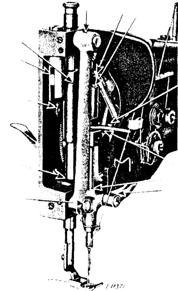
Fig. 4. Face Plate Removed, Showing Oiling Points
