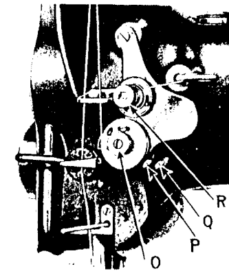
Fig. 18. Adjustment of Thread Controller
