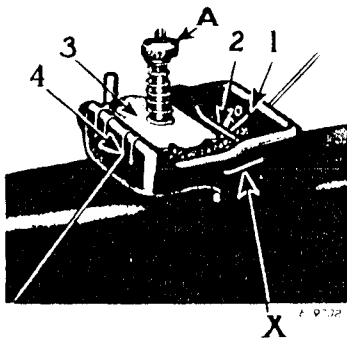
Fig. 13. Upper Threading
