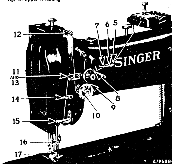
Fig. 14. Upper Threading
