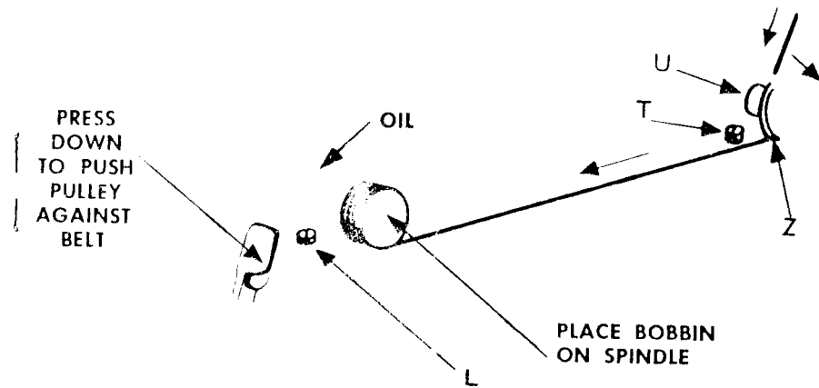
Fig. 15. Winding the Bobbin
