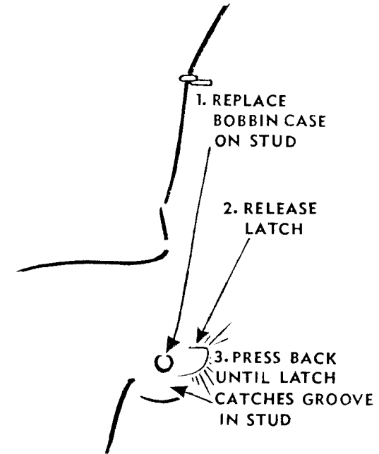
Fig. 19. Bobbin Case Threaded and Replaced
