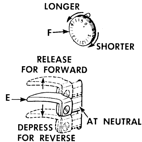
Fig. 27. Regulating Stitch Length on Machine 195K5
