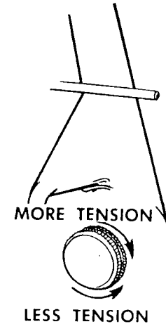
Fig. 24. Regulating Needle Thread Tension
