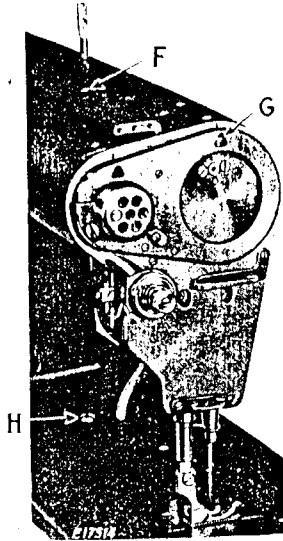
Fig. 19. Stitch Regulator and Indicator
