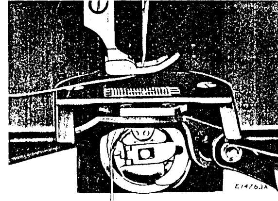
Fig. 10. Bobbin Case Threaded and Replaced
