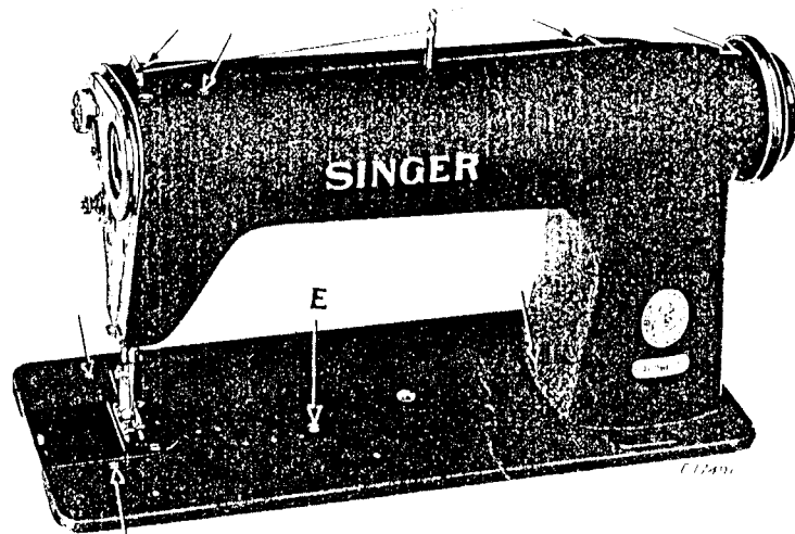
Fig. 3. Showing the Eight Oiling Points on the Machine
