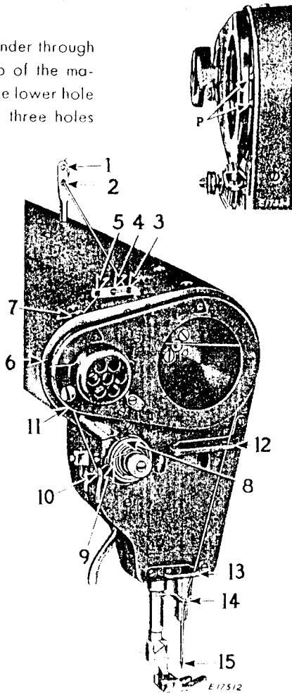
Fig. 11. Threading the Needle
