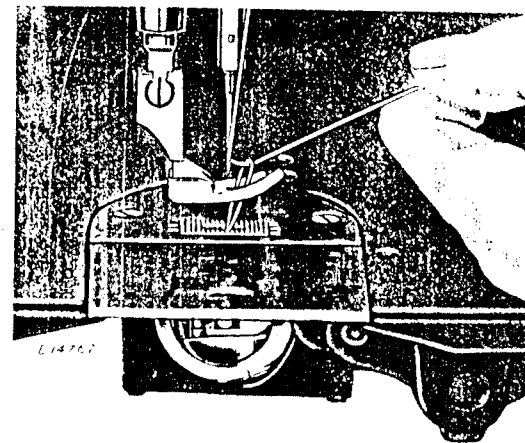
Fig. 12. Drawing Up the Bobbin Thread
