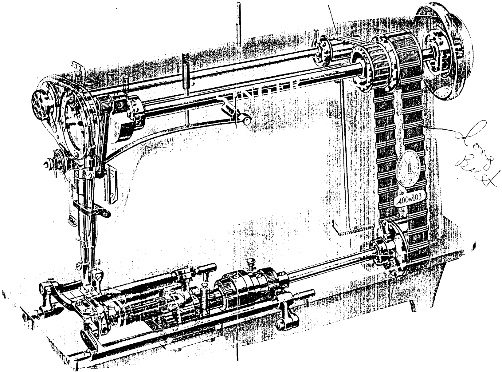
X-Ray View of 400w103 Machine (Lubrication Points Shown in Red)
