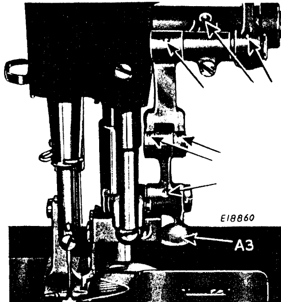
Fig. 33. Showing Trimmer Lever and Oiling Points for Trimmer Mechanism
