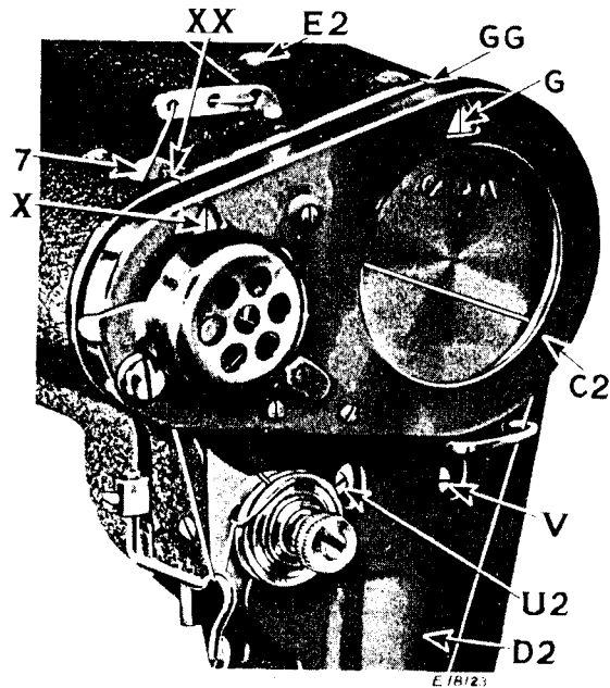
Fig. 20. Showing Timing Marks on Take-Up Discs and Face Plate
