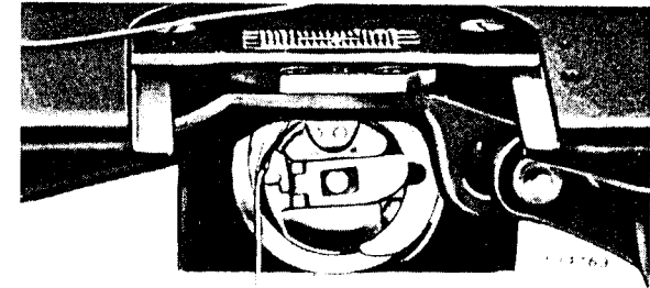
Fig. 10. Bobbin Case Threaded and Replaced
