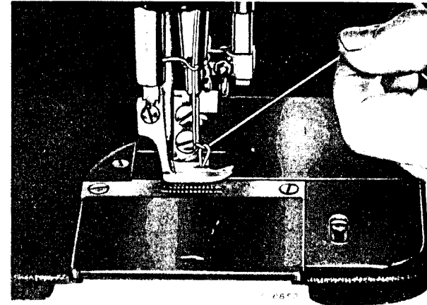
Fig. 12. Drawing Up the Bobbin Thread
