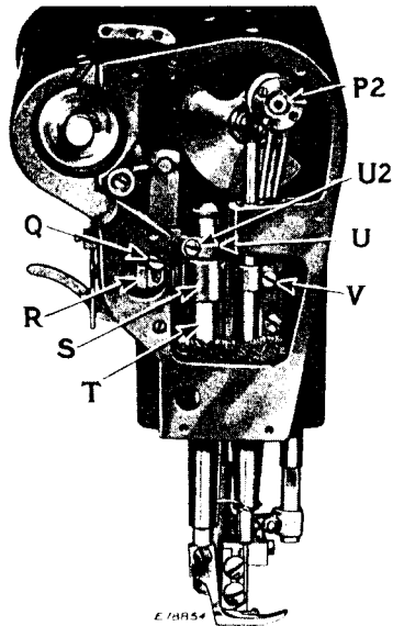
Fig. 22. Face Plate Removed
