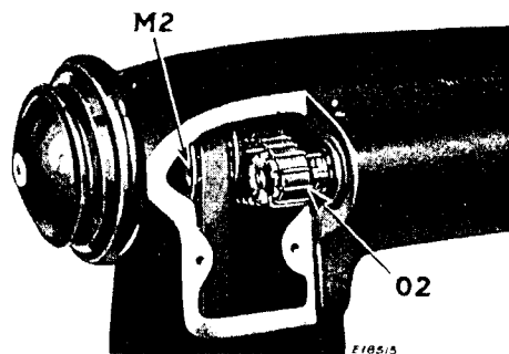
Fig. 30. Rear Arm Cover Removed
